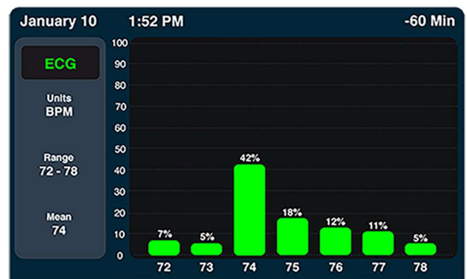
Histograma
